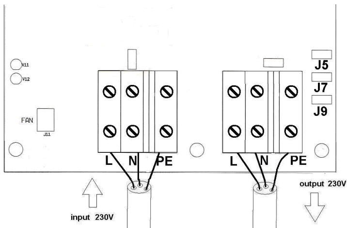
Figure 1: Input and output terminals
