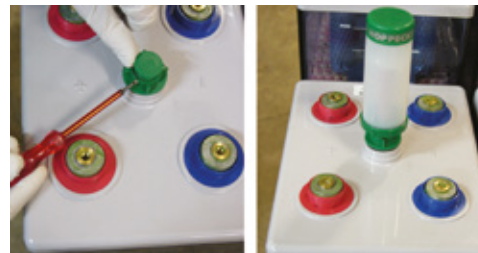
Fig. 5-14: Labyrinth plugs (left) and grid | aquagen recombination system (right)
